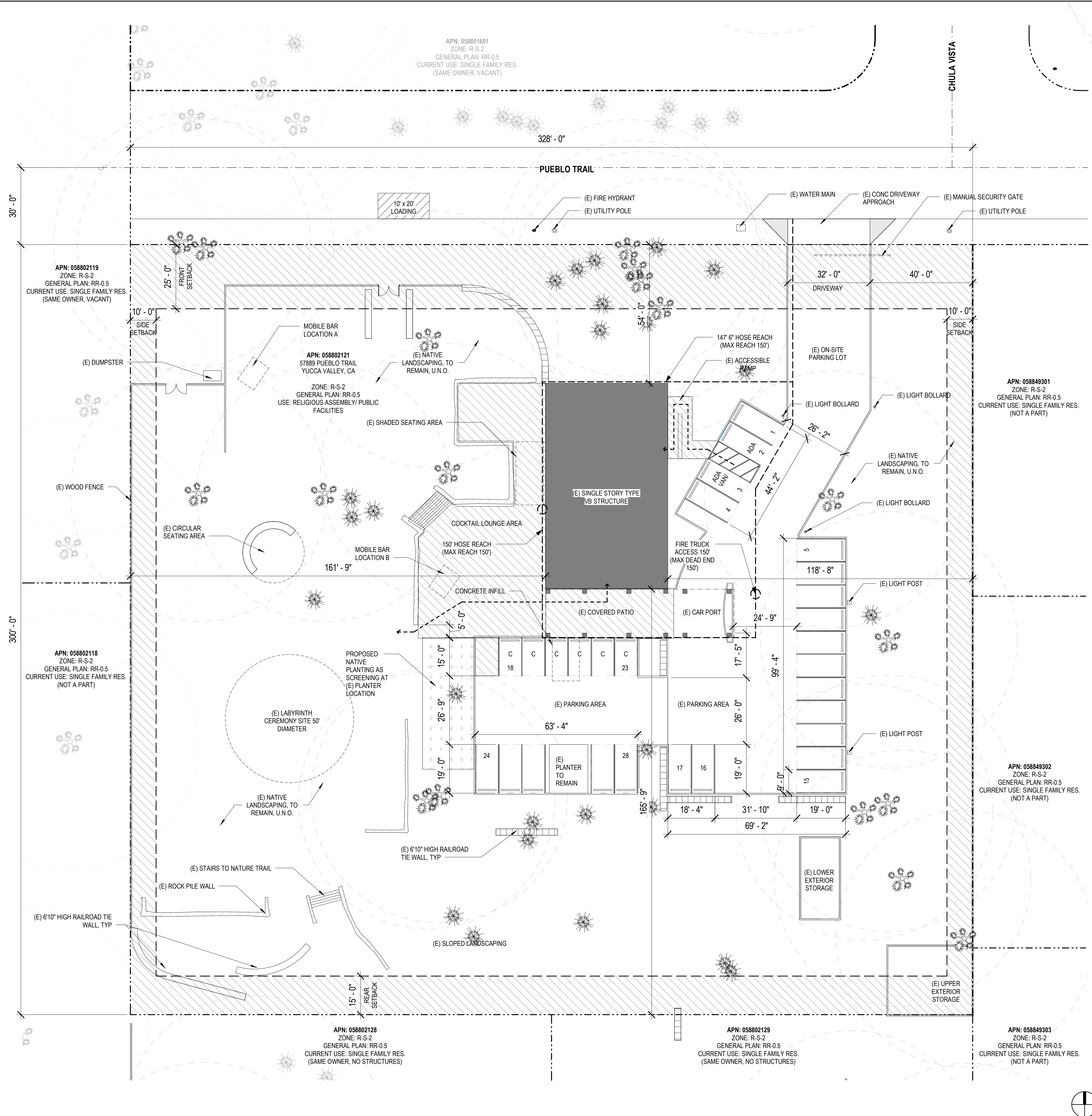
SITE PLAN - APN 058802121 1" = 20'-0"
