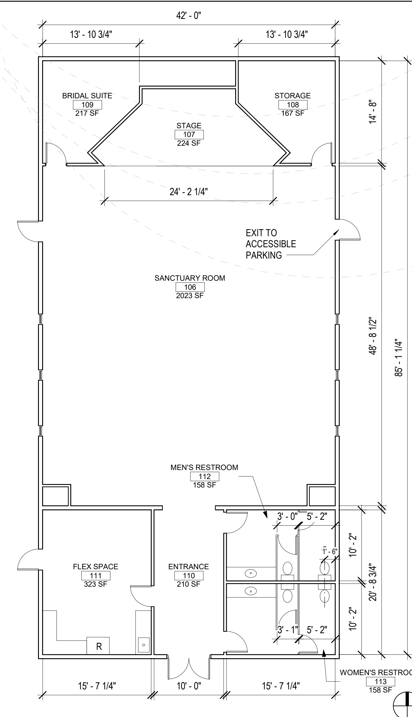
EXISTING FLOOR PLAN 1/8" = 1'-0"
